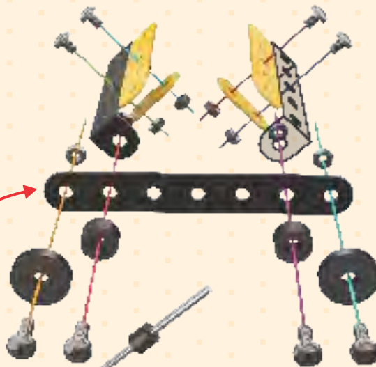
Small screw - 7pcs
