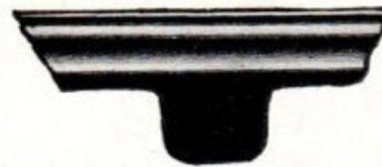
Cornice No. 11-B
