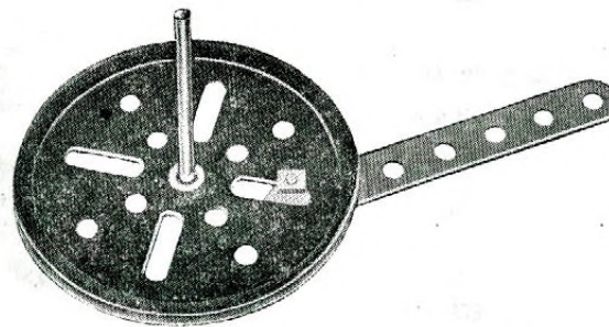
方帽的“扳牢”方法 Lock—Nutting 2 Nuts are used when some Parts require free Pivoting.
