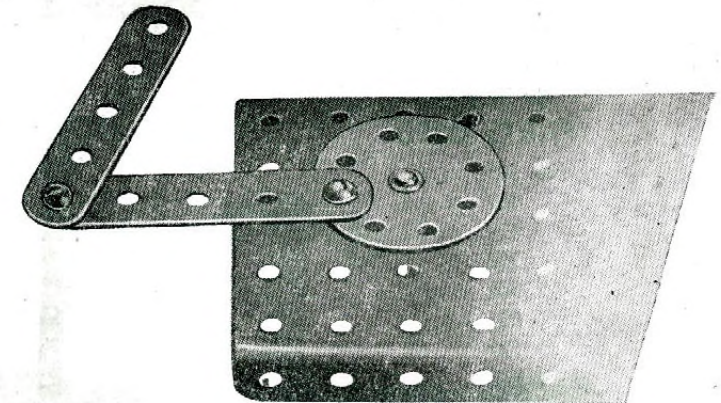
用有軸圓平輪代替轉輪 The Brush Wheel can be used as a Driving Wheel.
