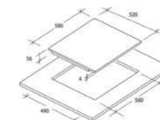
SCHEMA INDUCTION 60 CM
